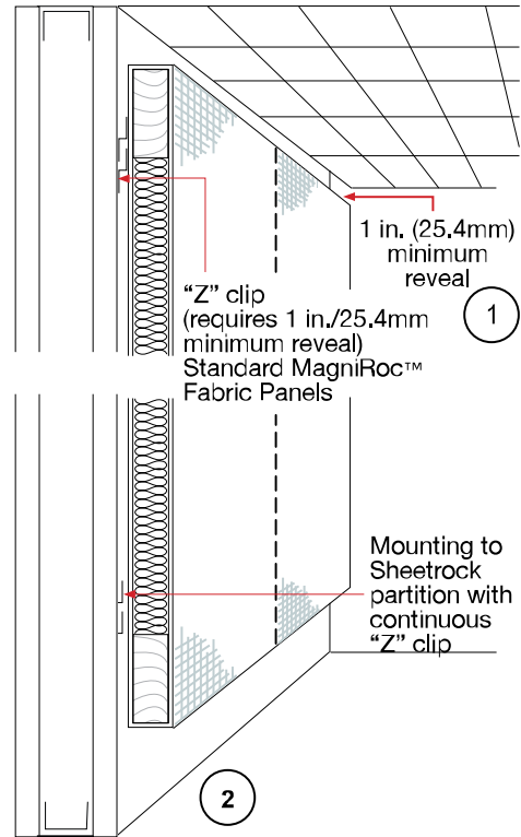
MagniRoc™ Fabric Panels mounted to single-layer Sheetrock
