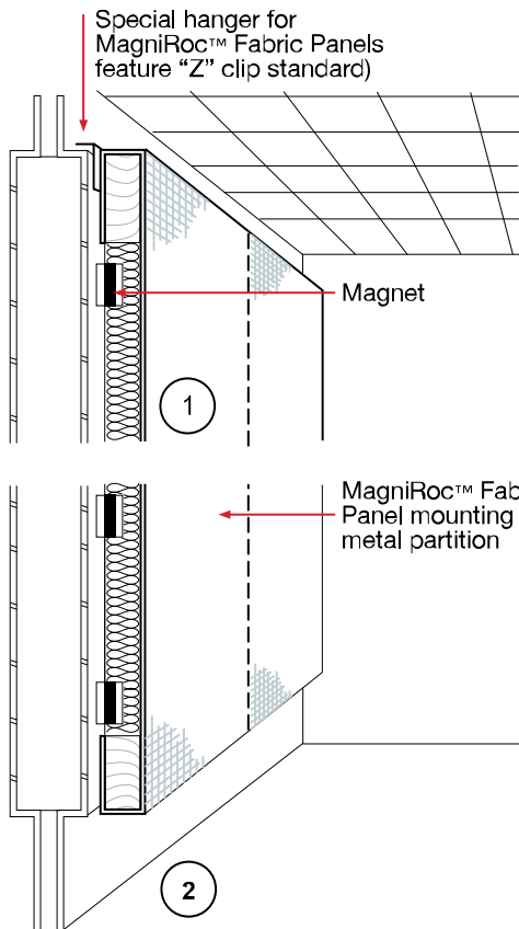
MagniRoc™ Fabric Panels with top angles mounted to metal partition
