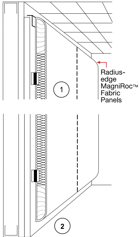
MagniRoc™ Fabric Panels 7/8 in. (22.2mm) radius double-layer Sheetrock with reveal
